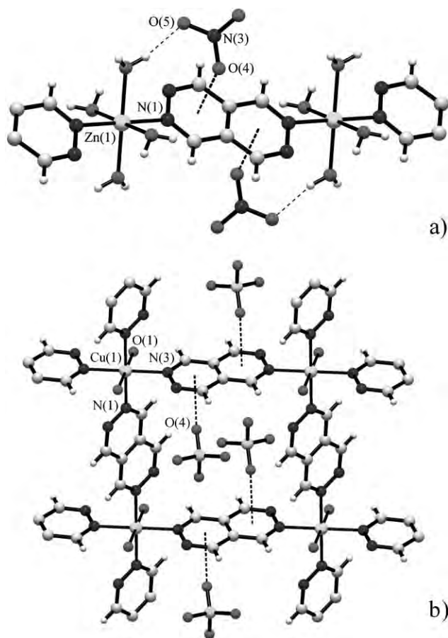
Fig. 1 a) 1D chain in complex 1 showing characteristic O \cdots\pi (2.875(2) Å) interactions with nitrate anions. b) Incorporation of ClO _4^- anions inside a rectangular cage in structure 3 and their interaction with \pi -systems.
